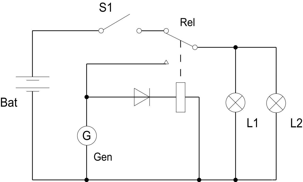
Fig 1 Lighting system
