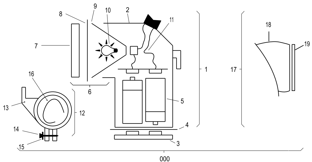
Fig 1 Light system
