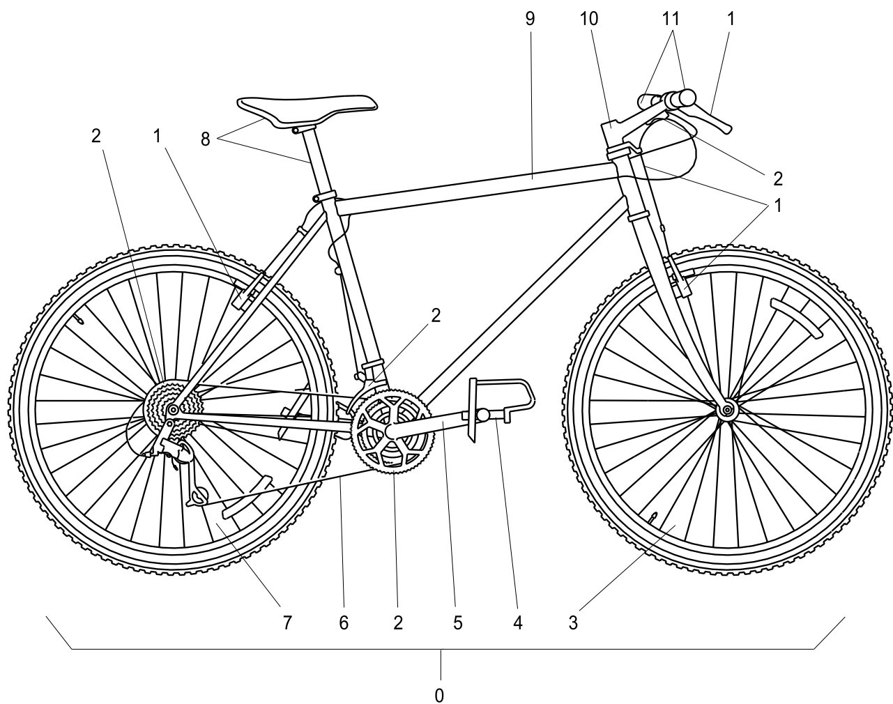
Fig 1 Complete bicycle
