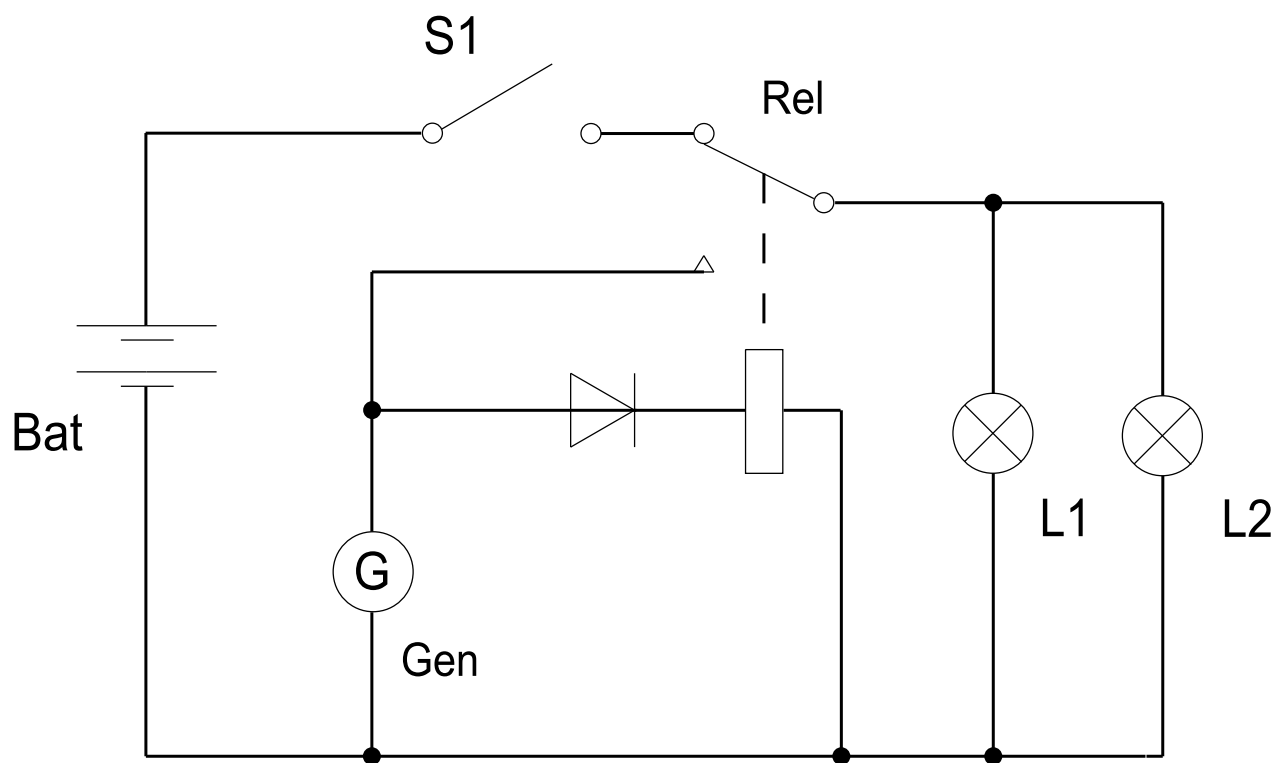
Fig 1 Lighting system
