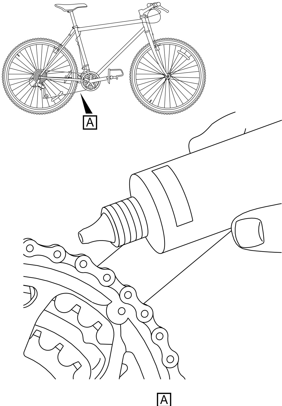
Fig 4 Lubricate the chain
